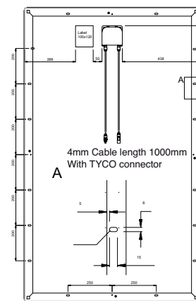
Rear side
